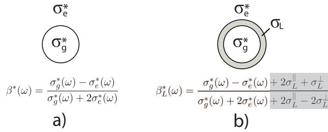
Figure 4.1: Dipolar coefficient for an uncharged grain (a) and a grain with conductive layer (b). The conductive layer conductivity \sigma_L can be decomposed into a parallel and perpendicular contributions ( \sigma_L^{\parallel} and \sigma_L^{\perp} ).
