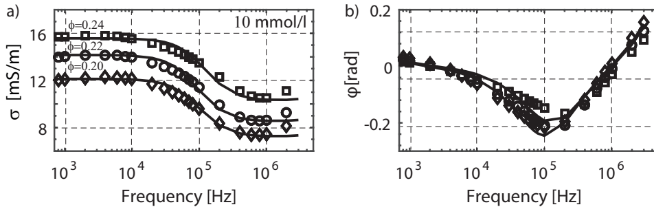
Figure 5.8: |\sigma| and \varphi spectra for 3 different electrode pairs, indicating differences in effective porosity in core B saturated with 10 mmol/l NaCl. The symbols represent the experimental data. Effective porosity is derived using the model in Section 5.3 (solid line).
