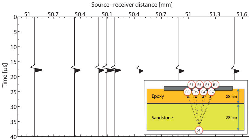
Figure 6.3: An example of the recorded common-source gather for the transmitted P-waves through the 2-layer sample.
