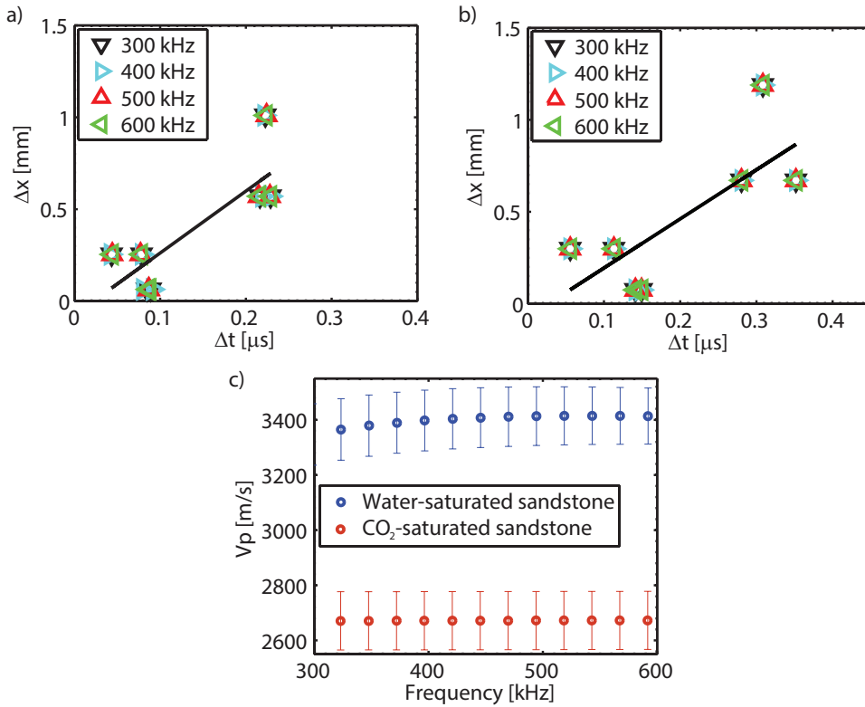
Figure 6.8: P-wave velocity estimation inside the sandstone layer. The best line fitting in a least-square sense for the water-saturated (a) and \text{CO}_2 -saturated (b) sandstone layers at P_p=77 bar and T=39^\circ\text{C} . c) The slope of the best-fit provides the estimates of V_p in the frequency range of 300-600 kHz.
