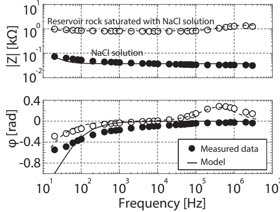
Figure 4.4: Magnitude |Z| and phase \varphi spectra of complex electrical impedance. Hollow circles show the impedance measurements of the reservoir rock, which is saturated with 170 mmol/l NaCl solution. Black circles show the impedance of the 170 mmol/l NaCl solution. Solid and dashed lines represent models given in Figure 4.2a and 4.2b, respectively. No adjustable parameters are required in both cases for the region representing bulk polarization (between 1 kHz and 20 kHz).
